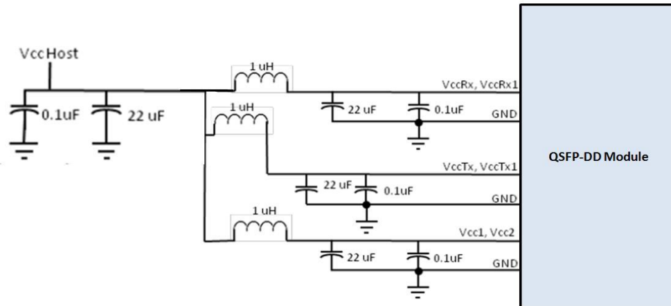
Figure 4.Recommended Power Supply Filter
