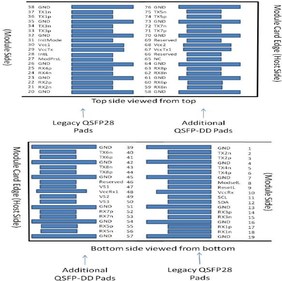
Figure 2. MSA Compliant Connector
