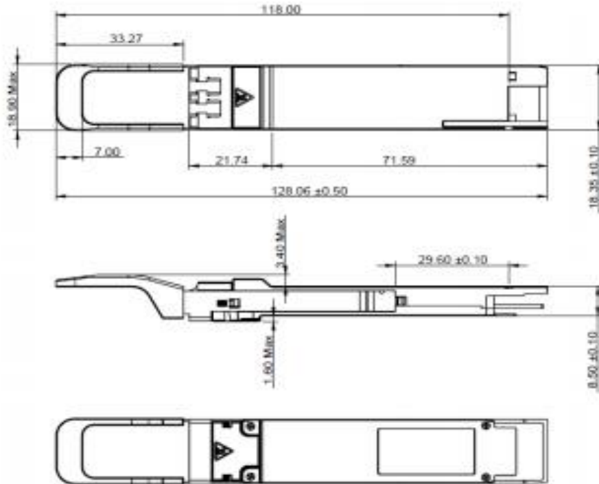
Figure 5. Mechanical Outline
