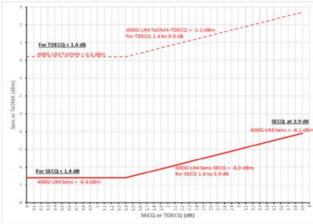
Figure 4. Illustration of Receiver Sensitivity Mask for 400G-LR4
