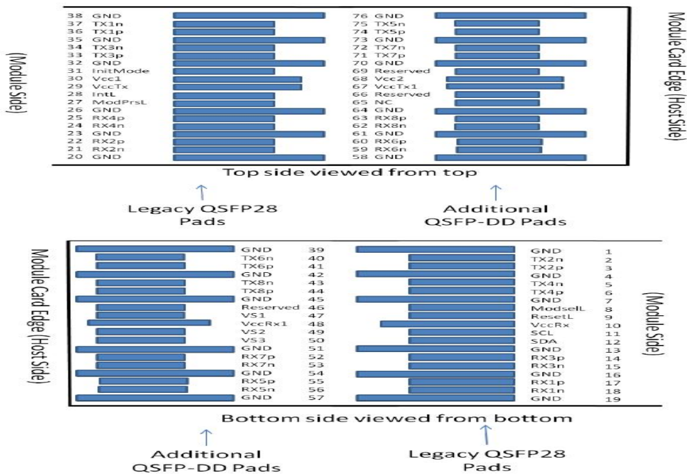
Figure 2. MSA Compliant Connector
